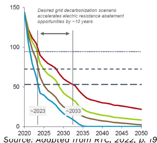
Figure 15: Conventional electric boiler emissions intensity v. fossil fuels (Kg CO 2 e/ MMBtu)
